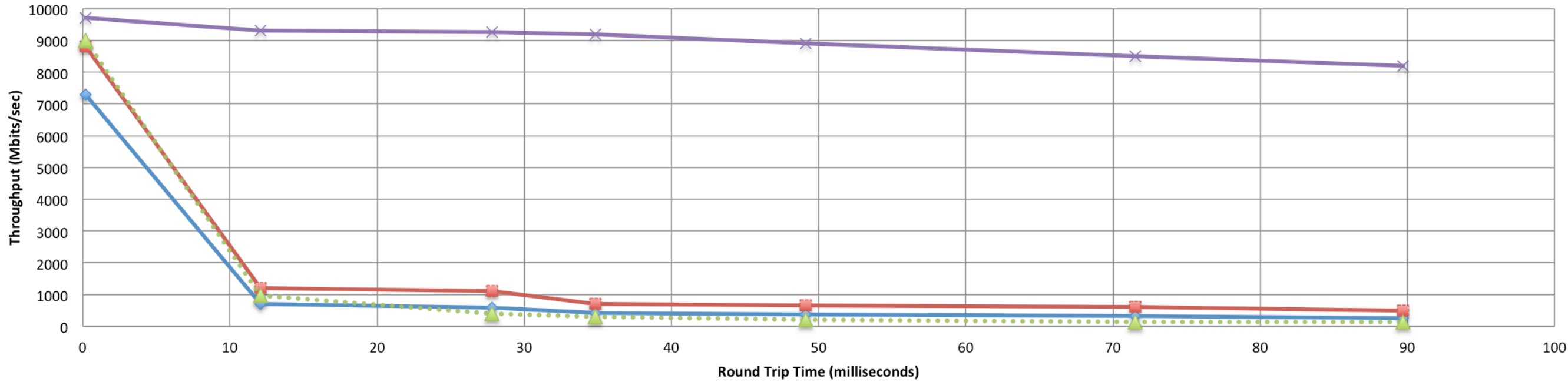
Throughput vs. Increasing Latency with .0046% Packet Loss
