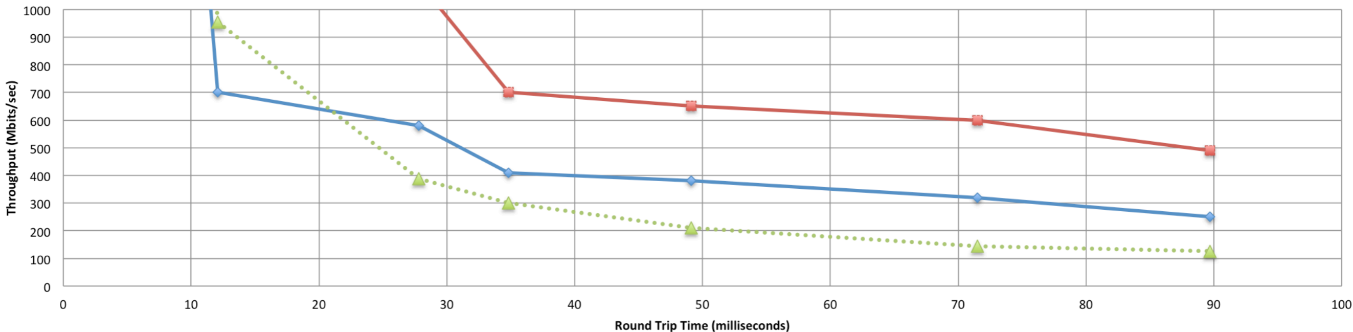
Throughput vs. Increasing Latency with .0046% Packet Loss (zoom of tail)
